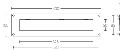
LSQ620
