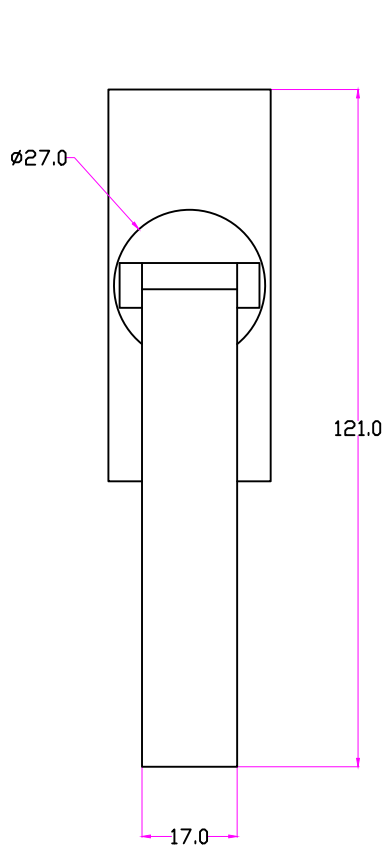
TOP VIEW
